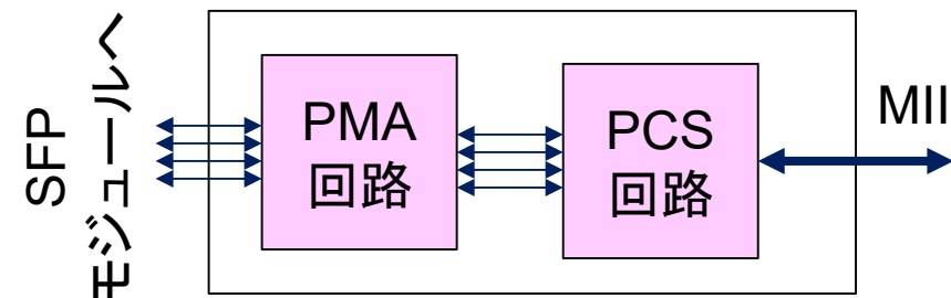
1000BASE-LX/SXのPHY
